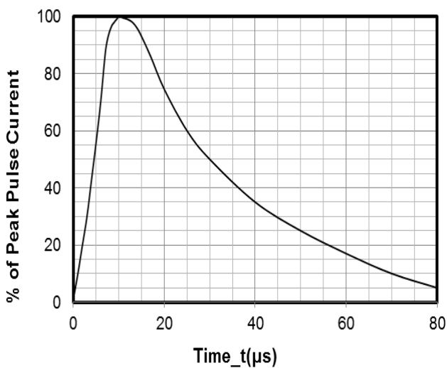
8 X 20 \mu s Pulse Waveform
